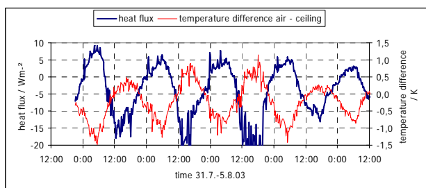
Figure 6: Measured heat fluxes and temperature differences between the room air measured 40 cm below the ceiling and the ceiling surface temperature.
