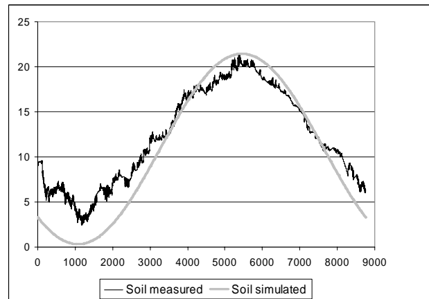
Figure 8 Measured and simulated soil temperature for the years 2001 (a), 2002 (b) and 2003 (c)
