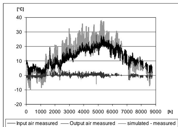
Figure 9 Inlet temperatures, outlet temperatures and simulation error of the Lamparter earth-air heat exchanger for the years 2001 (a), 2002 (b) and 2003 (c).
