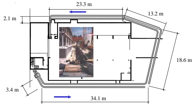
Figure 3: Outline of the Lamparter office building with earth-air heat exchanger.
