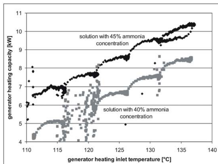
Fig. 4: Measured generator heating capacity versus generator heating inlet temperature (at two different ammonia solution concentrations).
