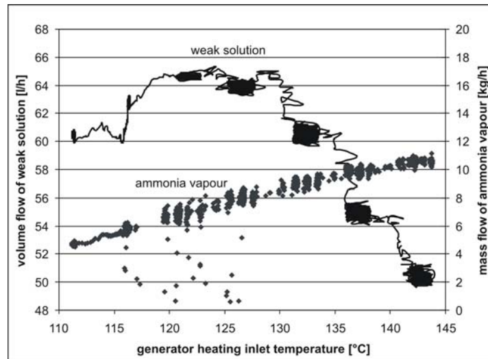
Fig. 3: Measured volume flow of weak solution and mass flow of ammonia vapour versus generator heating inlet temperature (generator B II).
