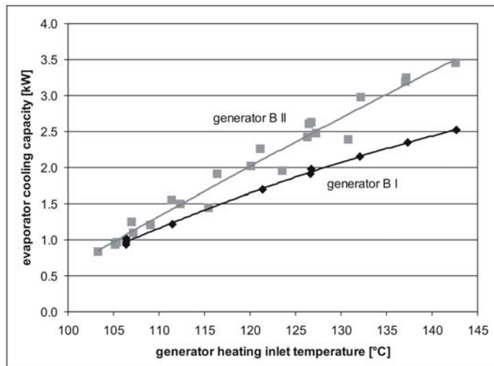
Fig. 6: Measured evaporator cooling capacity versus generator heating inlet temperature (in dependence of the generator heat transfer surfaces).
