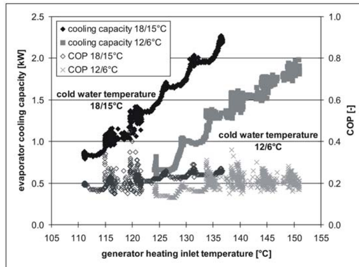
Fig. 2. Measured evaporator cooling capacities and COPs of the DACM versus generator heating inlet temperatures and evaporator temperatures of 18/15°C and 12/6°C, respectively.
