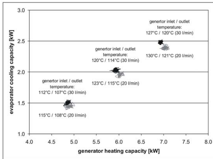
Fig. 5: Measured evaporator cooling capacity versus generator heating capacity (at different external heating volume flows, generator B II).
