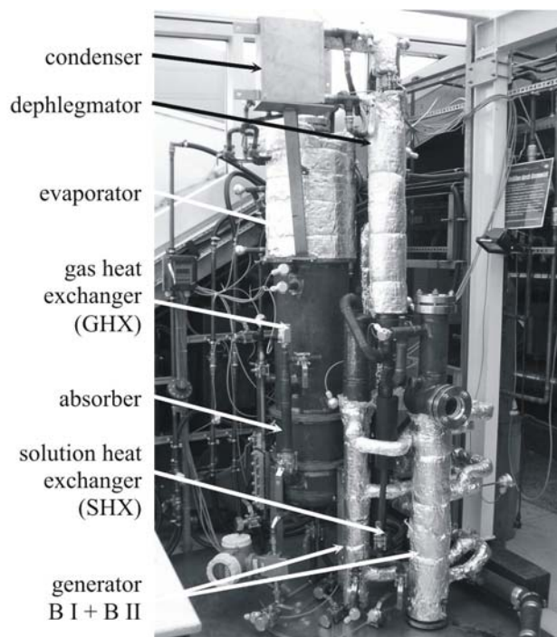
Fig. 1: DACM prototype (photo: zafh.net)
