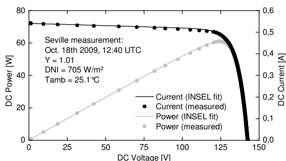
FIGURE 8: The measured IV values (dots) in this plot were gathered outdoors, with UF close to 1. This particular IV curve has been fitted with a two-diode model using the INSEL PV simulation software (lines).
