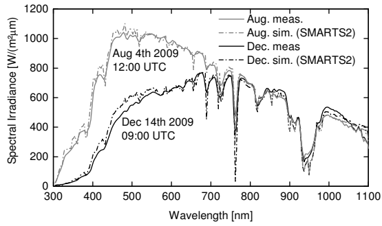
FIGURE 3: Measured (solid lines) and SMARTS2 simulated (dashed lines) spectra.
