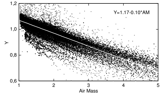
FIGURE 4: All Y values measured in Seville throughout 2009 (gray and black dots) plotted against AM. For the linear fit only the Y values measured at DNI > 500 W/m 2 were considered (black dots).
