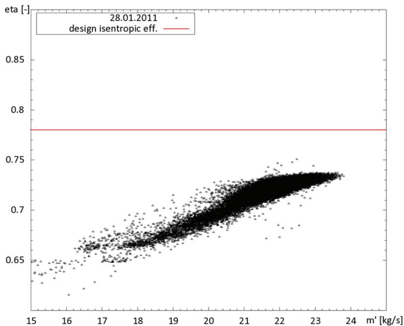
Figure 5: Isentropic efficiency of turbine versus fluid mass flow
