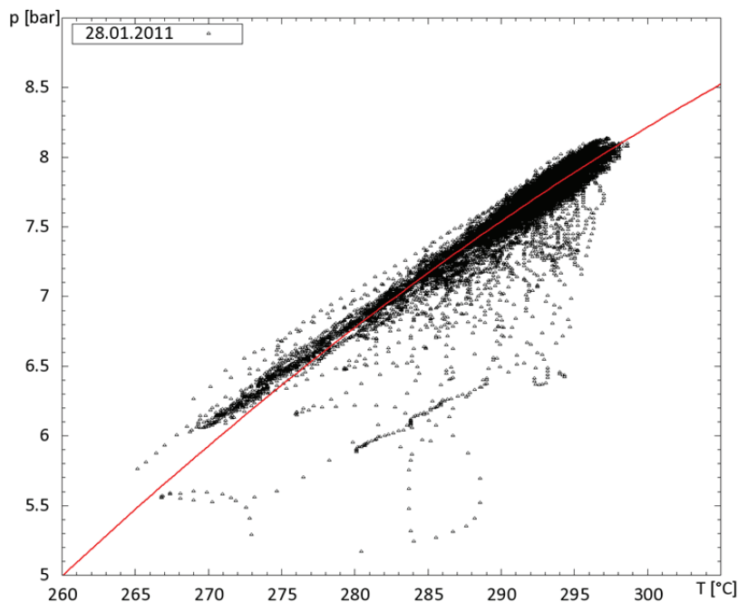
Figure 4: Evaporator behaviour
