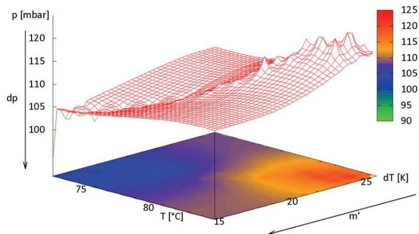
Figure 8: Condenser pressure vs. sink temperature and temperature spread
