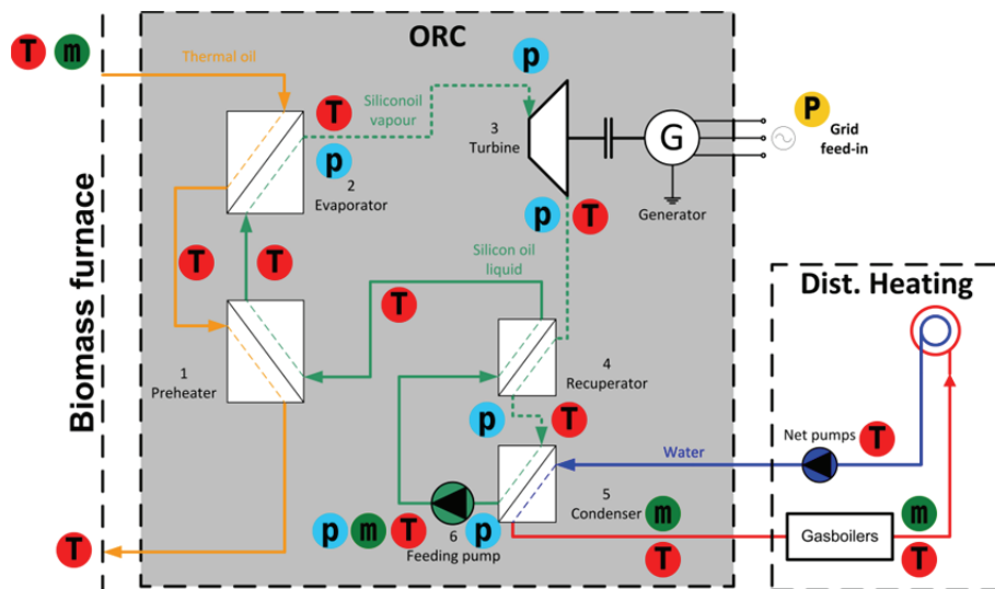
Figure 2: Scheme of the of the OR-Cycle including sensors and gauges [ERHART]
